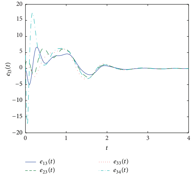
FIGURE 3: The error states of complex network e_{i3} .
