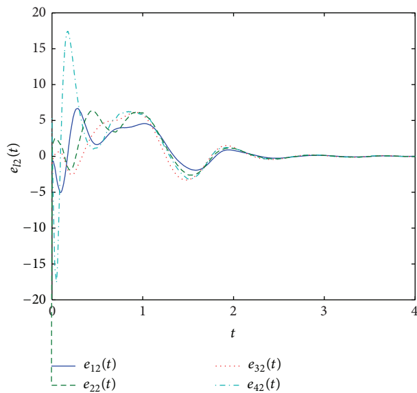
FIGURE 2: The error states of complex network e_{i2} .
