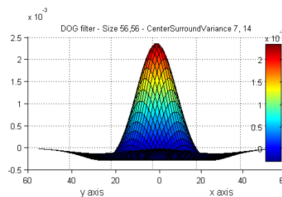
Figure 3: Difference of Gaussian filter with sigma of 7 for the centre and 14 for the surround. Kernel size is 56×56.
