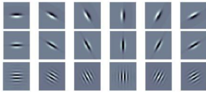
Figure 1: One sample scale of 6 oriented filter banks shown for (top) DoG, (middle) LoG, and (bottom) Gabor wavelet.
