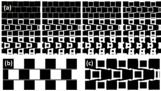
Figure 7: Café Wall results with centre/surround/window in the ratio 1:2:3. (a) Multiscale output result for scale varying from fine to coarse scale starting from the centre Gaussian \sigma of 1 (top-left), increasing 1 pixel at a time to 12 pixels (bottom-right). Original image for the Café Wall illusion (b) with enlarged output (c) for \sigma = 6 .
