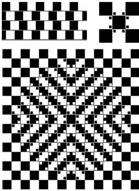
Figure 4: Investigated patterns (top): Café Wall, simple bulge Checkerboard, and (bottom) Complex bulge pattern (Akiyoshi Kitaoka)- http://www.ritsumei.ac.jp/~akitaoka/index-e.html
