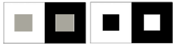
Figure 6: (left) SBC (Simultaneous Brightness Contrast) illusion, where identical gray test patches appear with misperception of brightness, and (right) Irradiation pattern where equal sized black and white test patches appear with the misperception of size.
